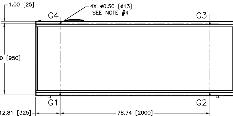
ANCHOR BOLT & ISOLATOR MOUNTING LOCATIONS
