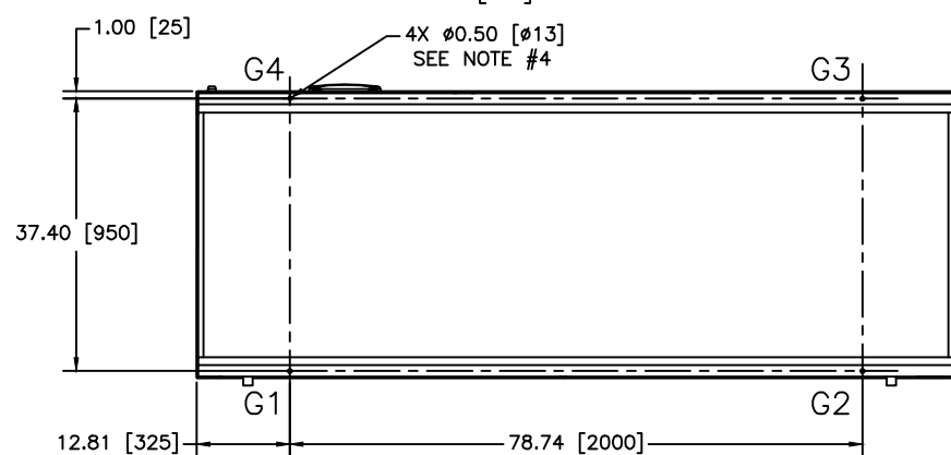
ANCHOR BOLT & ISOLATOR MOUNTING LOCATIONS
