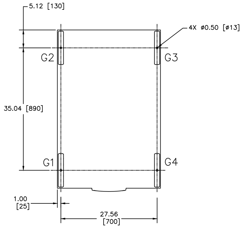
ANCHOR BOLT & ISOLATOR MOUNTING LOCATIONS
