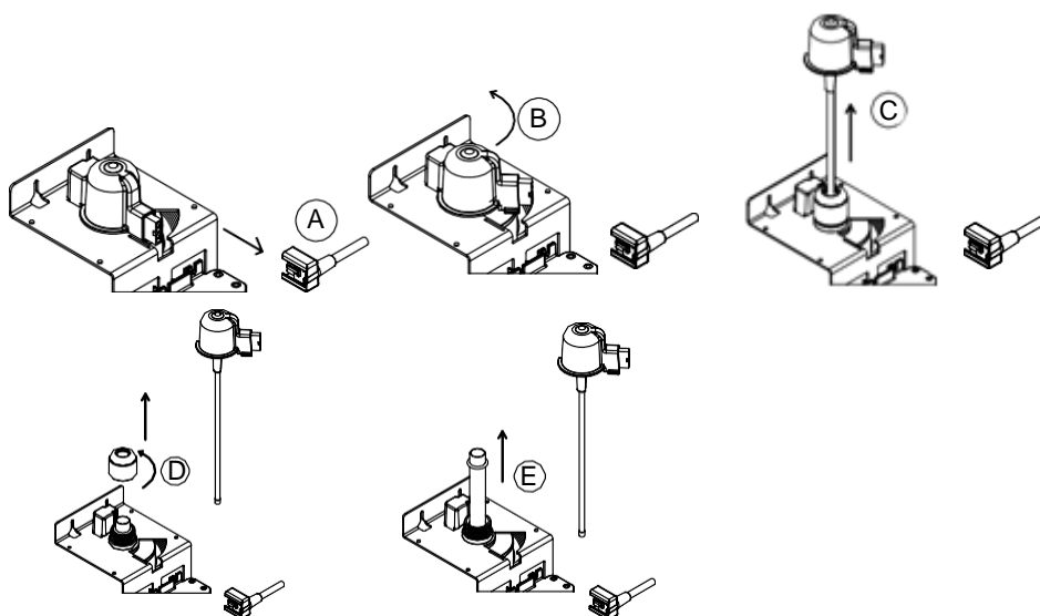
Figure 6-1 Lamp and Quartz Sleeve Replacement
