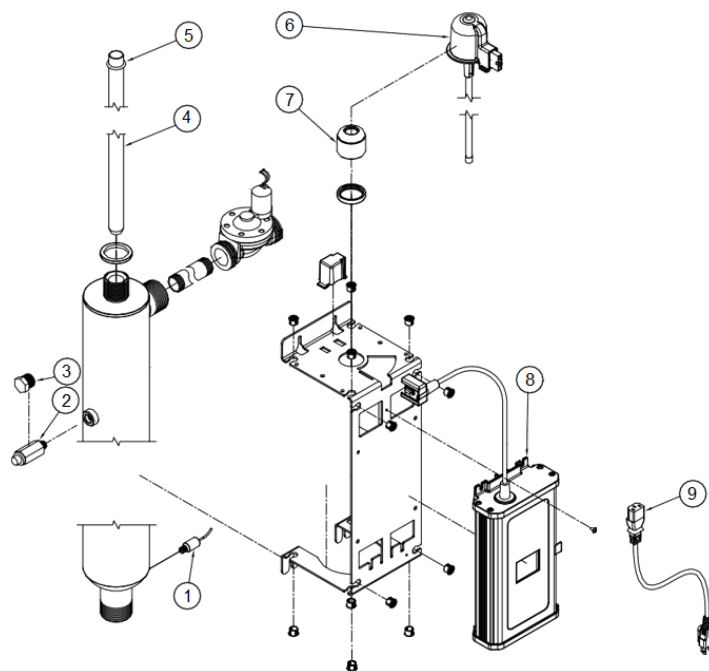
Figure 5-3 Lync UV Parts
