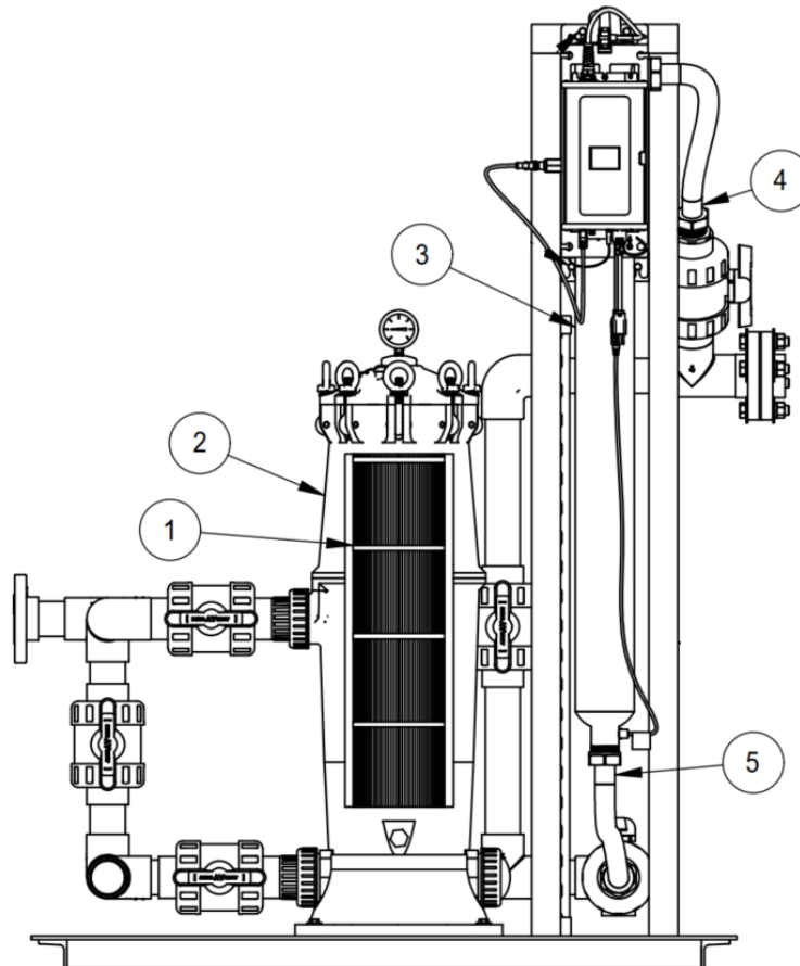
Figure 5-1 WQ-UV Skid Parts
