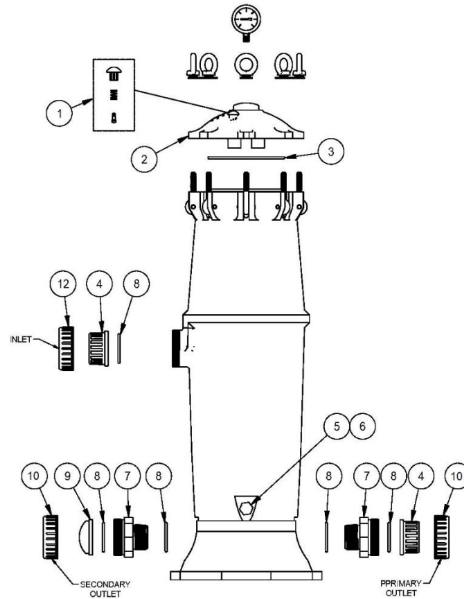
Figure 5-2 Lync Cartridge Filter Parts
