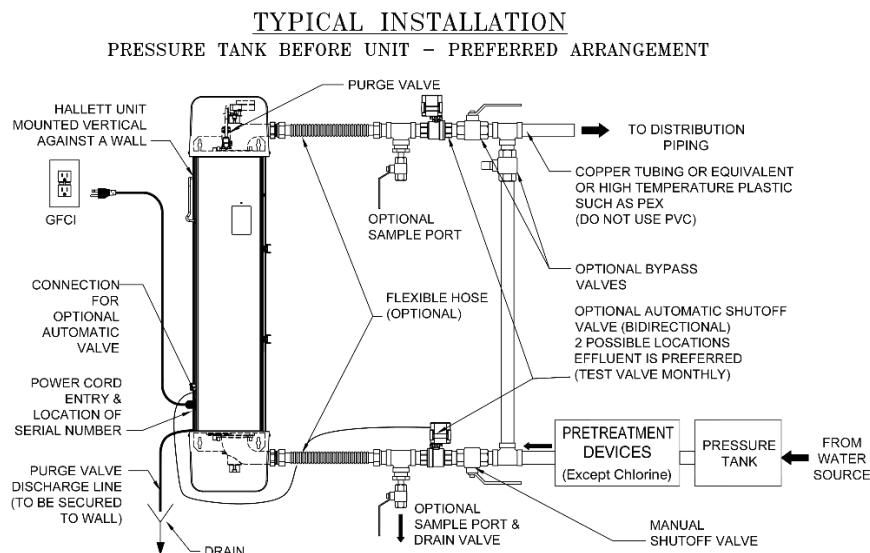
Figure 4-2: Typical Installation, Preferred Arrangement
