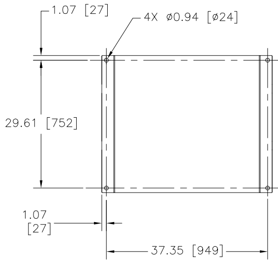
ANCHOR BOLT LOCATIONS
