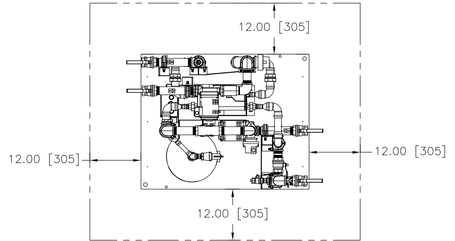
RECOMMENDED CLEARANCE
