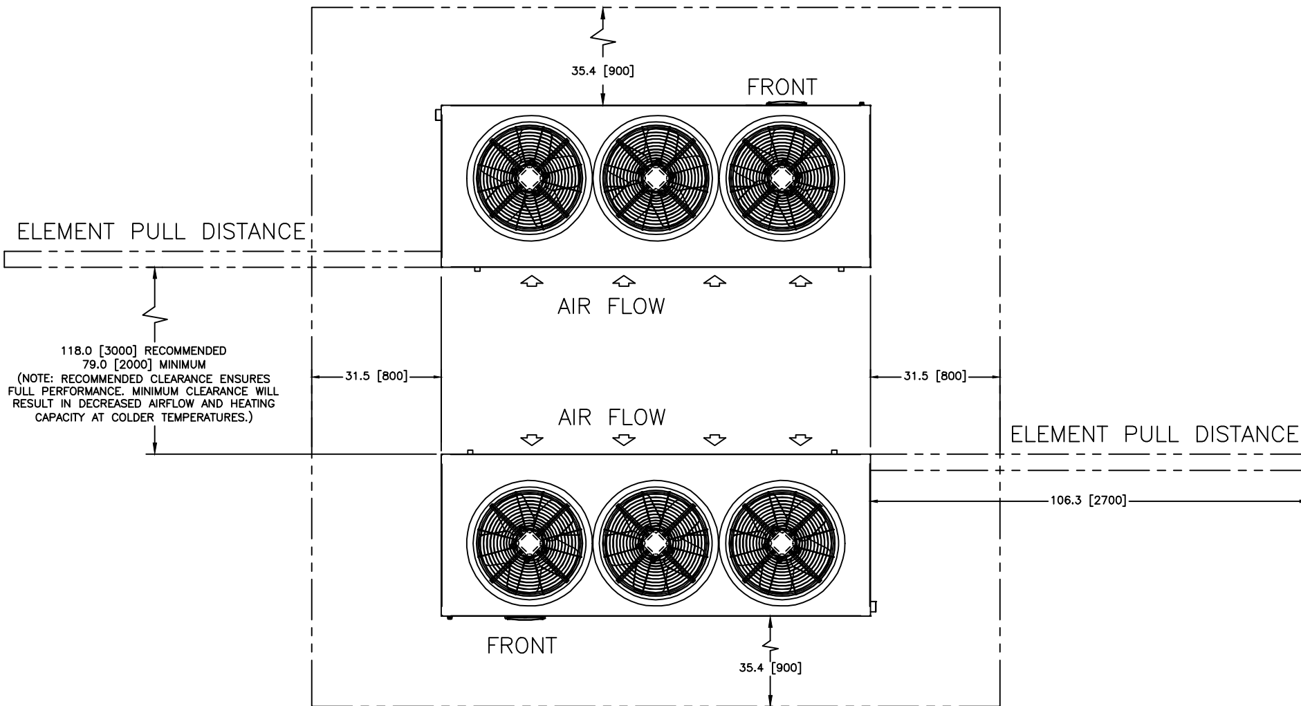
SHOWN TOP VIEW BACK-TO-BACK UNITS
