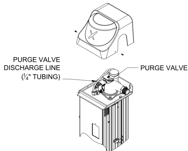
Figure 3-1 Lync UV-H Header Connections
